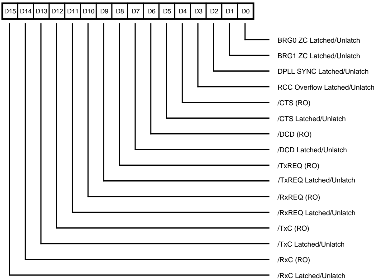
Figure 61. Miscellaneous Interrupt Status Register (MISR)
