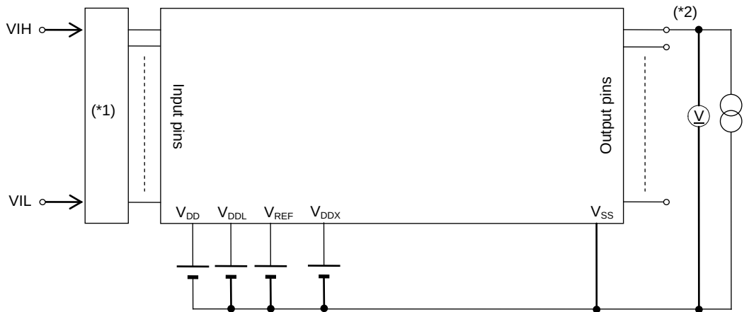
Measuring circuit 2
