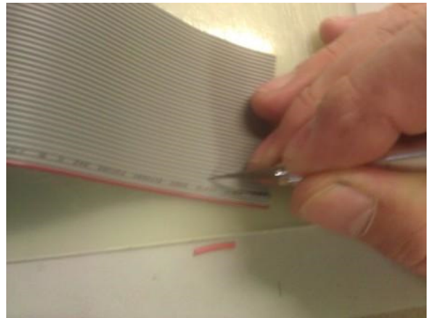
Step 2 Cut Ribbon Cable to Desired Width
