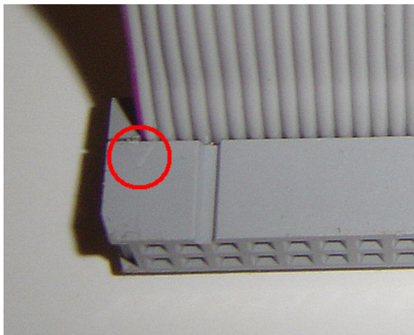
Step 3 Place IDC Connector on the cable and close it all the way to assure proper connection
