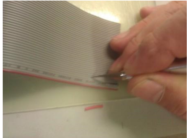
Step 2 Cut Ribbon Cable to Desired Width
