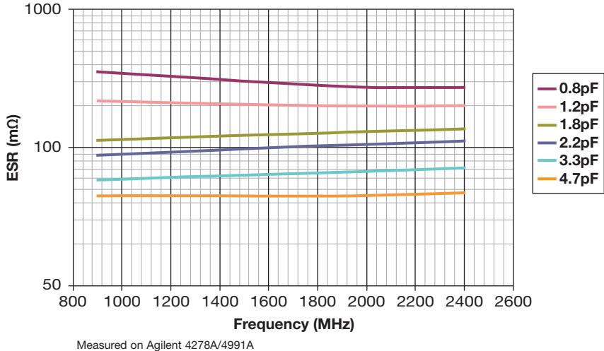
Accu-P® 0402 Typical ESR vs Frequency
