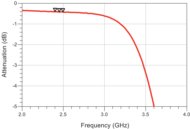
LOW BAND INSERTION LOSS
