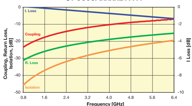
CP0603AxxxxBNTR
