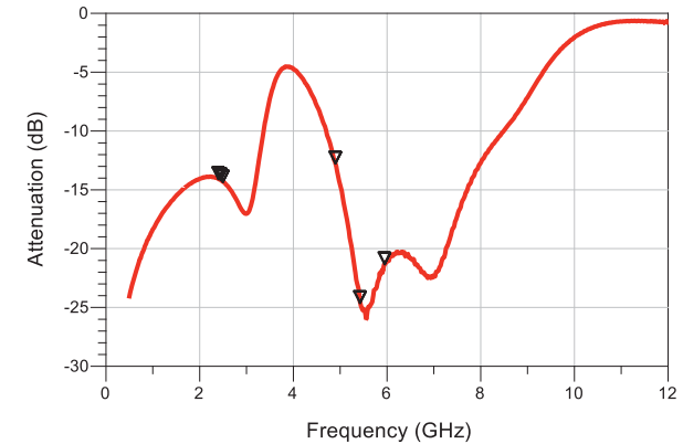
COMMON PORT RETURN LOSS
