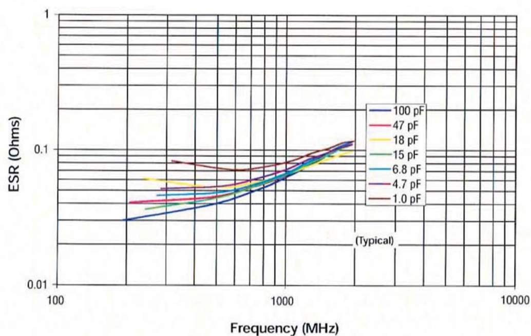
UQ CS ESR vs. Frequency
