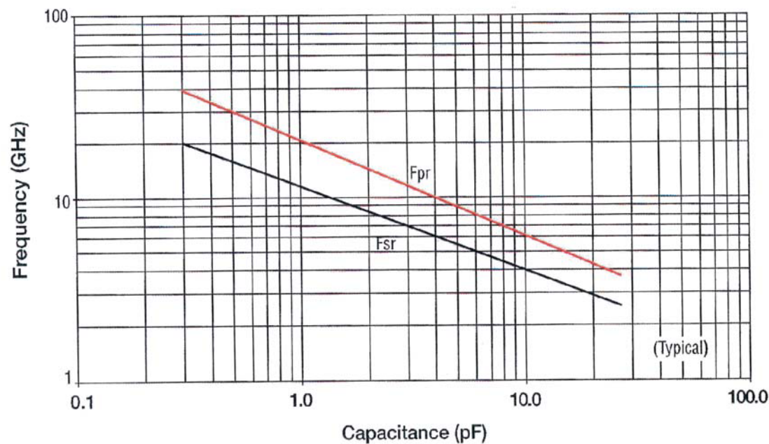
UQ CL Resonance Frequency
