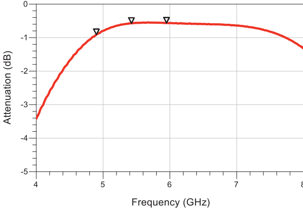
HIGH BAND INSERTION LOSS
