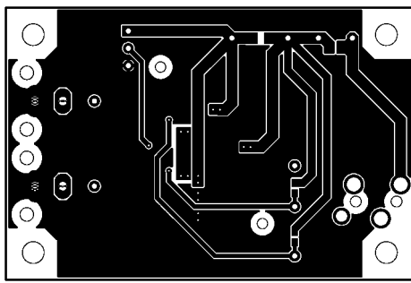
(BOTTOM LAYER – TOP VIEW)
