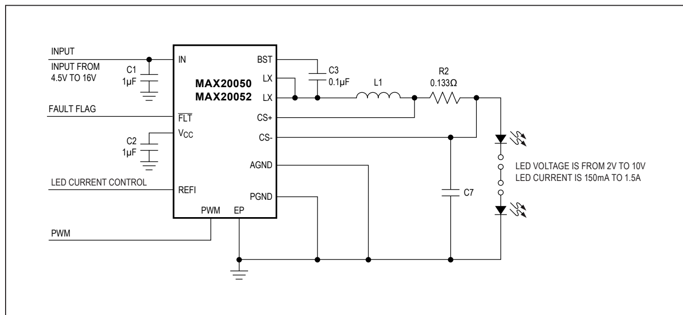
Figure 4. Typical Input Voltage (12V)
