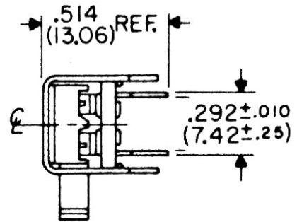
TWO POLE
