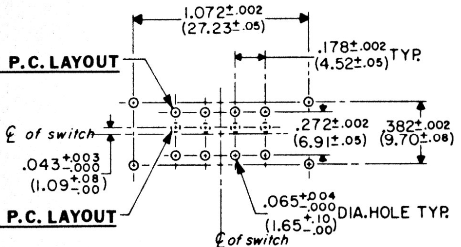
TWO POLE
