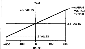
TRANSFER CHARACTERISTICS AT V_s=5.0 VDC
