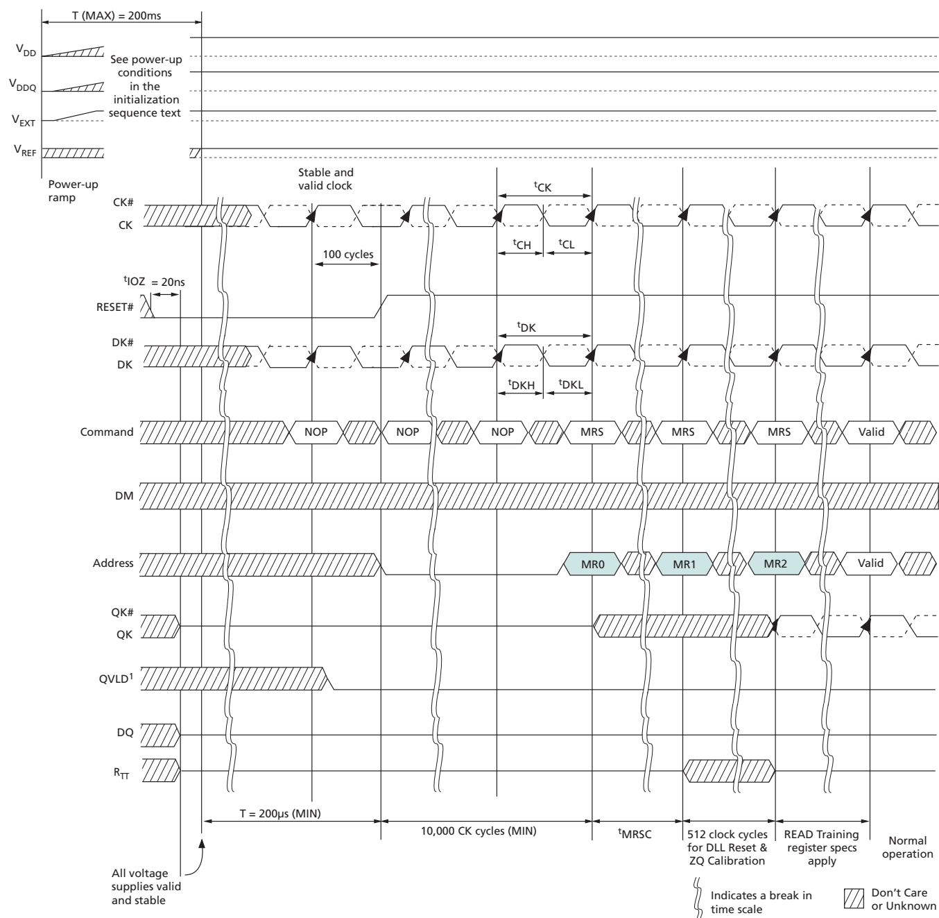
Figure 41: Power-Up/Initialization Sequence
