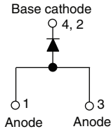
TO-247AC
