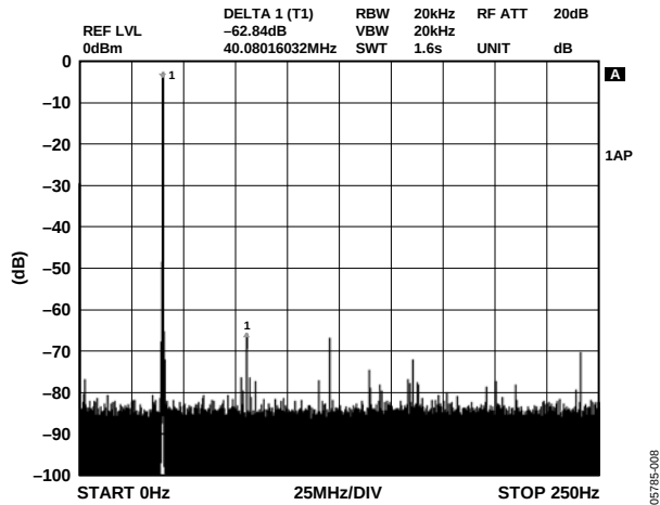
Figure 8. f_{OUT} = 40.1 MHz, f_{CLK} = 500 MSPS, Wideband SFDR
