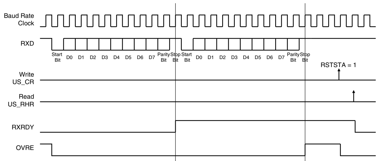
Figure 33-21. Receiver Status
