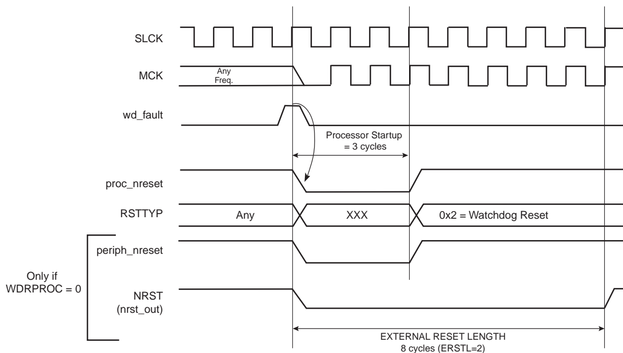
Figure 12-8. Watchdog Reset
