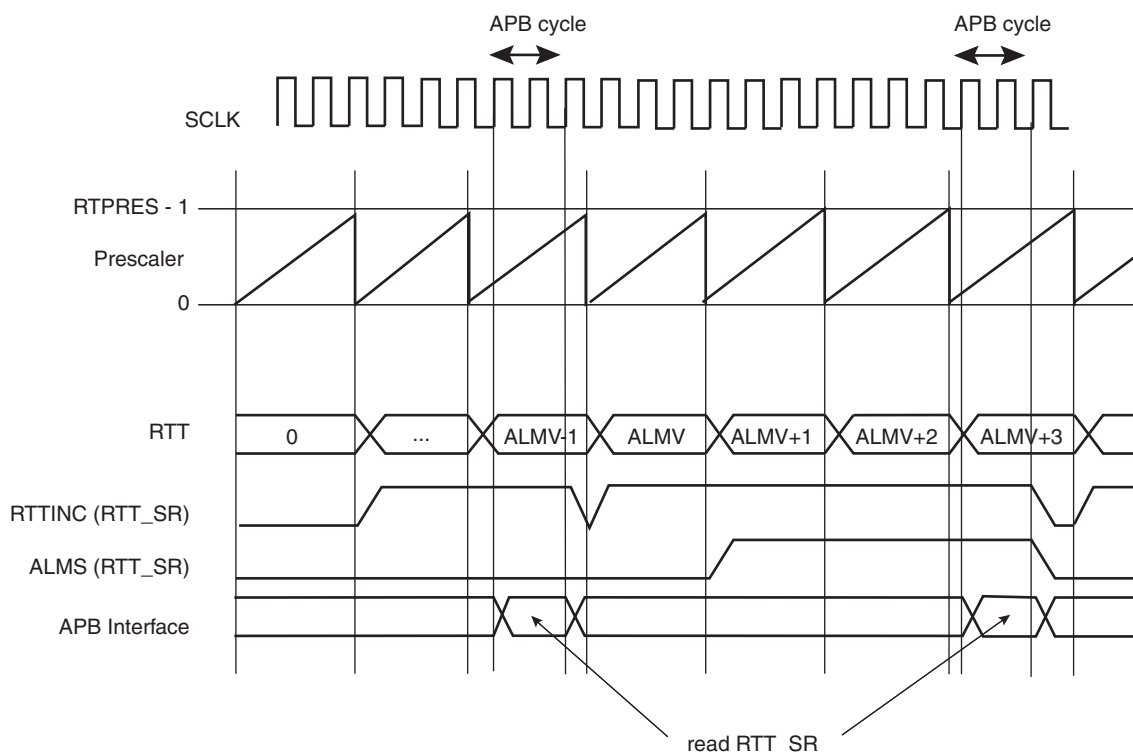
Figure 13-2. RTT Counting
