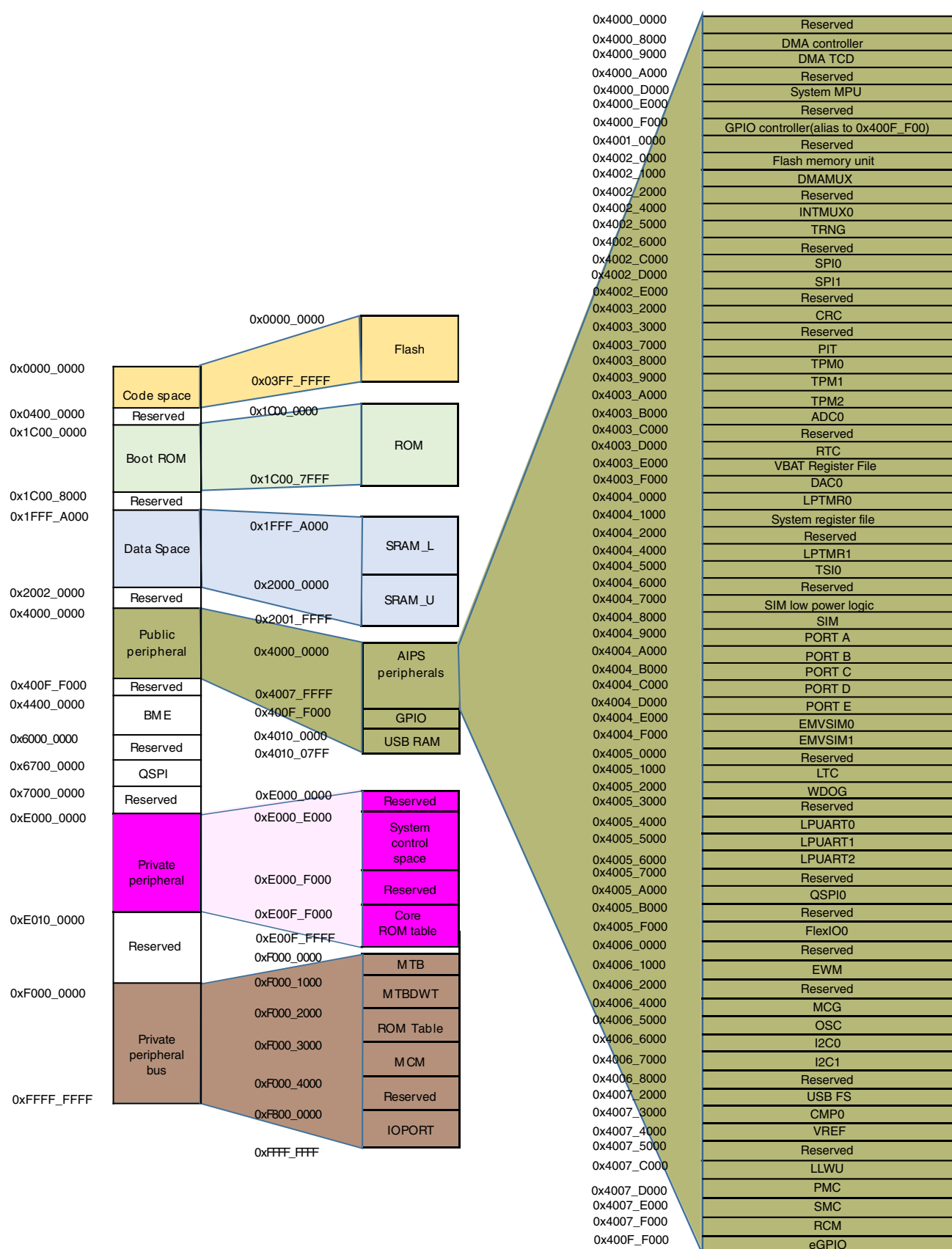
Figure 4. Memory map
