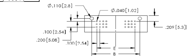
P.C. BOARD PATTERN
