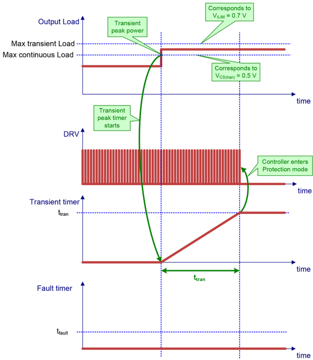
Figure 73. Too Long Transient Peak Power Delivery
