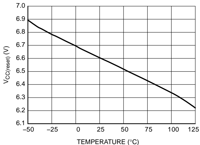
Figure 36. V_{CC} Decreasing Level at Which the Internal Logic Resets V_{CC(reset)}
