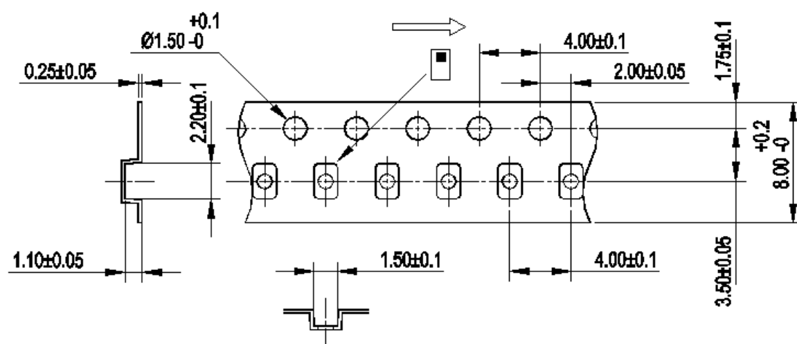
Carrier Tape
