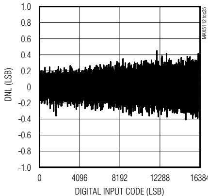
OP6 DIFFERENTIAL NONLINEARITY vs. DIGITAL INPUT CODE
