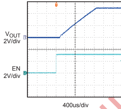
Turn on Delay and Rise Time No Cdv/dt, C OUT =10uF, no load
