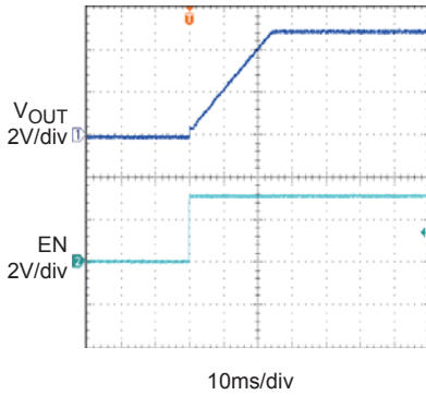
Turn on Delay and Rise Time Cdv/dt=1nF, C OUT =10uF, no load
