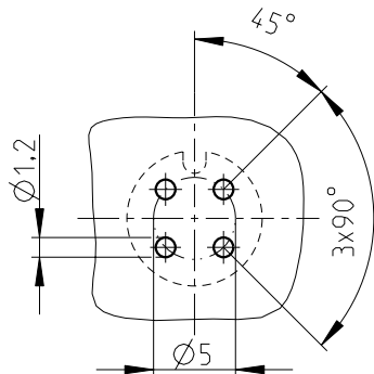
PCB-Layout (advice)
