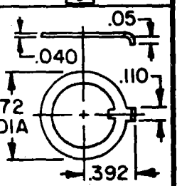
LOCKING RING
