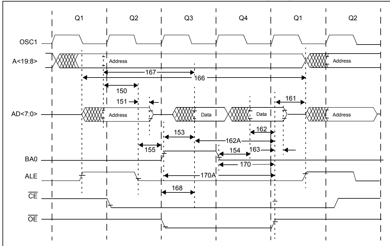
FIGURE 27-6: PROGRAM MEMORY FETCH TIMING DIAGRAM (8-BIT)
