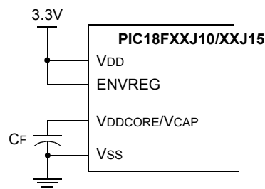
FIGURE 24-2: CONNECTIONS FOR THE ON-CHIP REGULATOR
