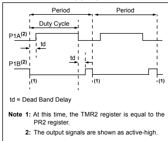
FIGURE 18-4: HALF-BRIDGE PWM OUTPUT
