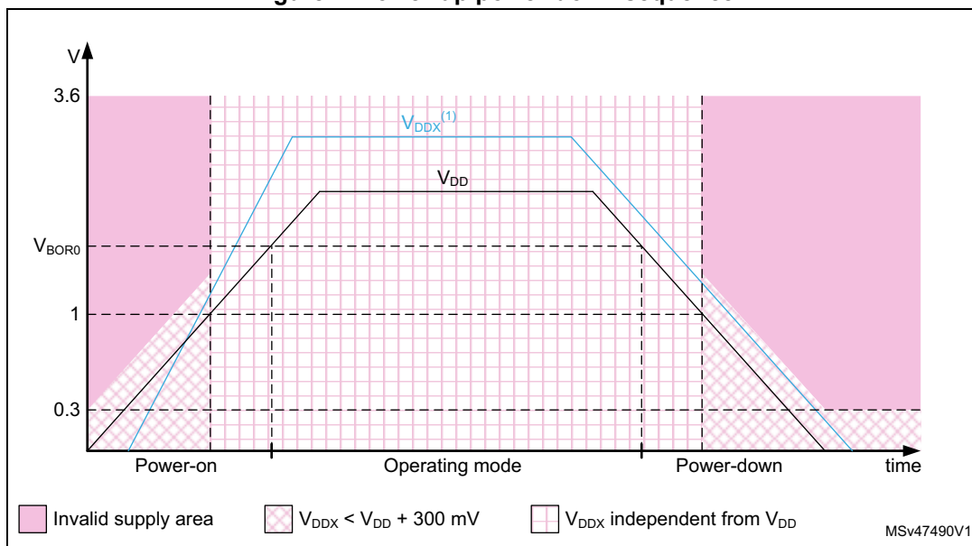
Figure 4. Power-up/power-down sequence
