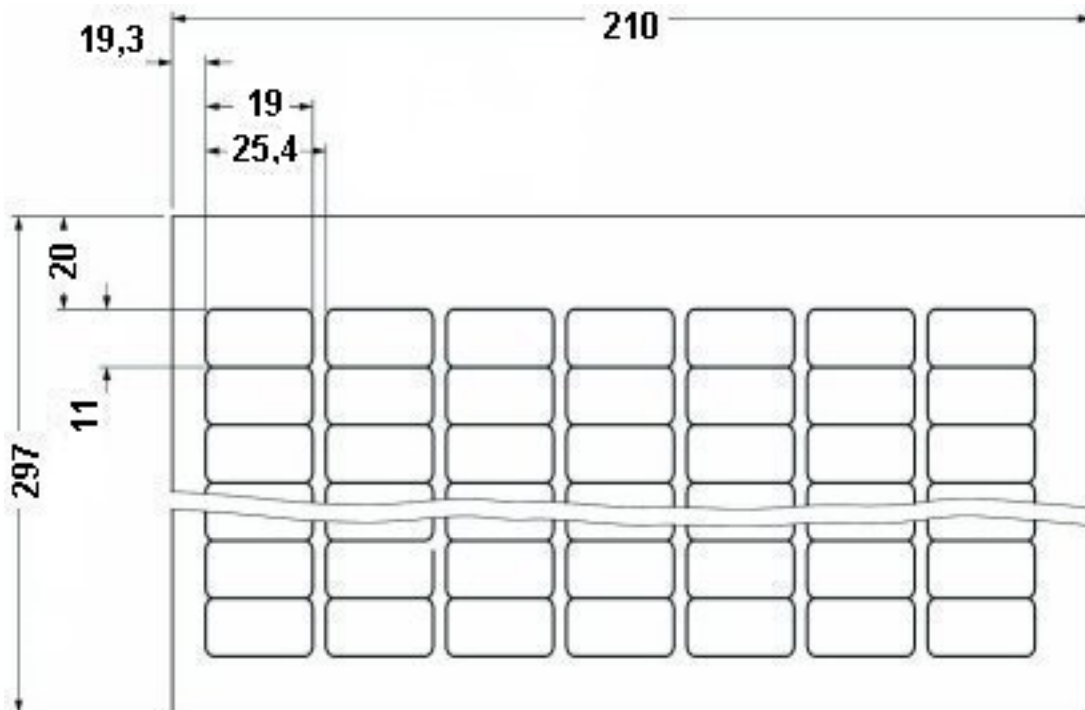
Dimensioned drawing
