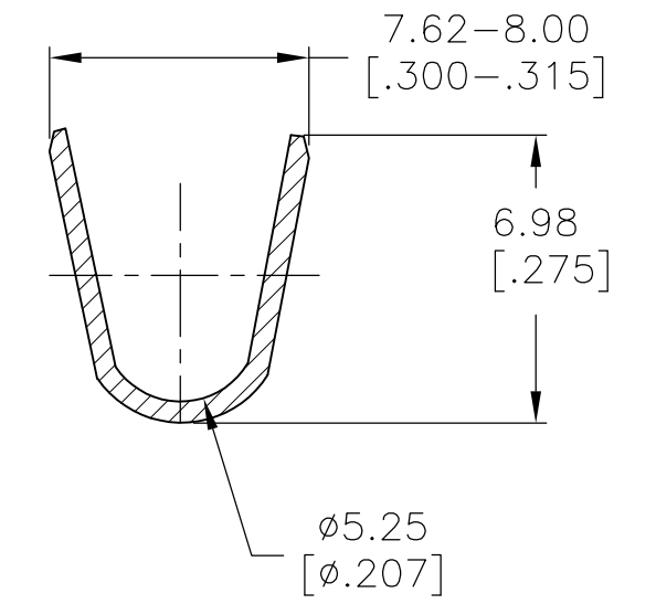
INSULATION RANGE [0.160-.210] SECTION, A-A
