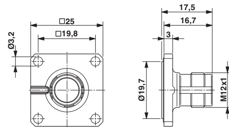
M12 flush-type plug, square flange
