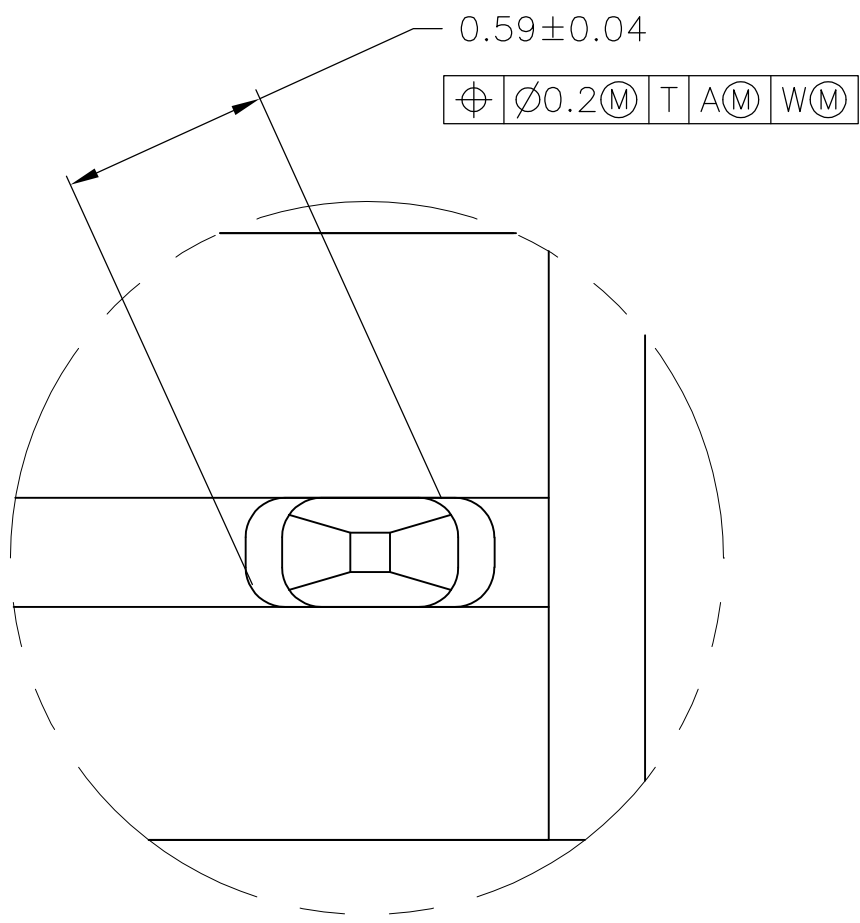
DETAIL Z SCALE 10:1
