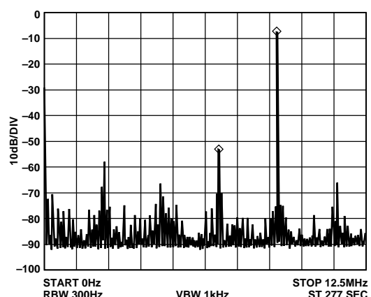
Figure 20. f_{MCLK} = 25 MHz, f_{OUT} = 9.1 MHz, Frequency Word = 5D2F1AA0
