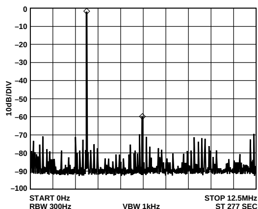
Figure 14. f_{MCLK} = 25 \text{ MHz} , f_{OUT} = 3.1 \text{ MHz} , Frequency Word = 1FBE76C9
