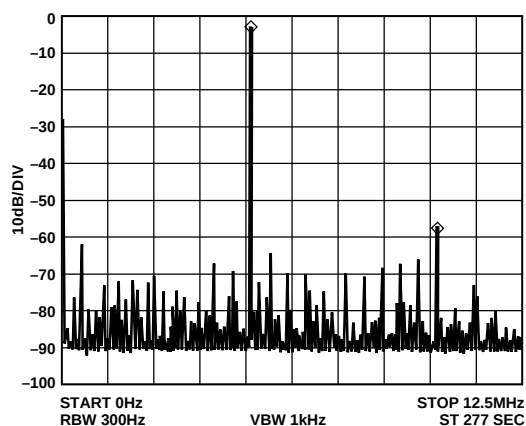
Figure 16. f_{MCLK} = 25 \text{ MHz} , f_{OUT} = 5.1 \text{ MHz} , Frequency Word = 34395810
