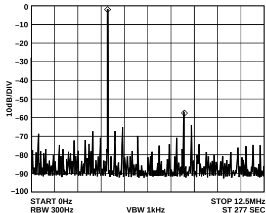
Figure 15. f_{MCLK} = 25 \text{ MHz} , f_{OUT} = 4.1 \text{ MHz} , Frequency Word = 29FBE76D
