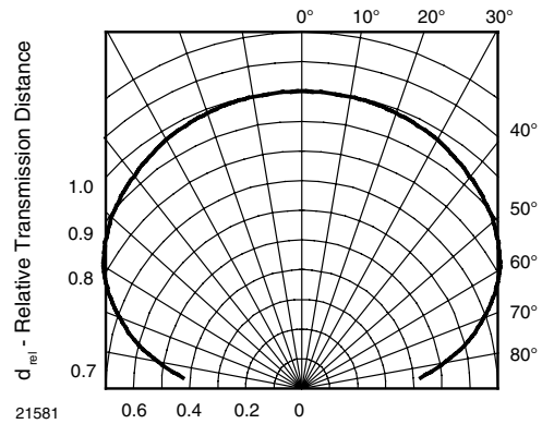
21581 Fig. 12 - Horizontal Directivity
