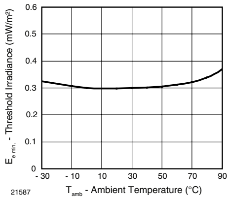
21587 T_{\text{amb}} - Ambient Temperature ( ^{\circ}\text{C} ) Fig. 10 - Sensitivity vs. Ambient Temperature
