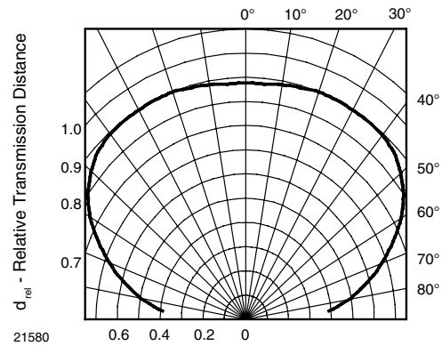
21580 Fig. 13 - Vertical Directivity
