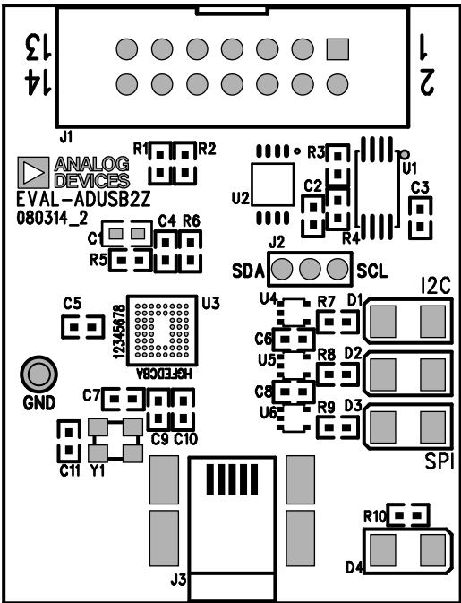
Figure 28. Board Layout—Top View
