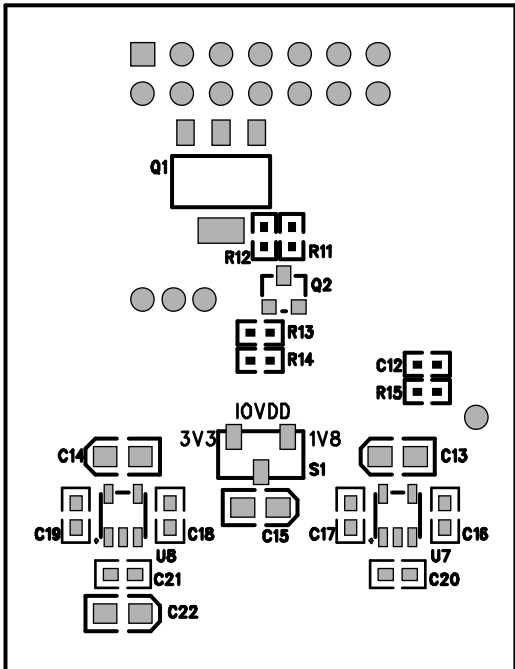
Figure 29. Board Layout—Bottom View
