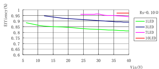
Efficiency vs. No. of LEDs L=47\mu\text{H} , R_s=0.10\Omega\text{hm}
