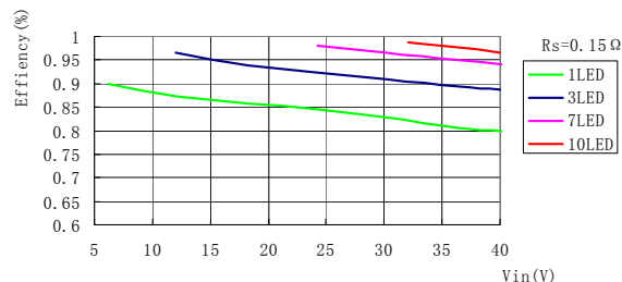
Efficiency vs. No. of LEDs L=47\mu\text{H} , R_s=0.15\Omega\text{hm}
