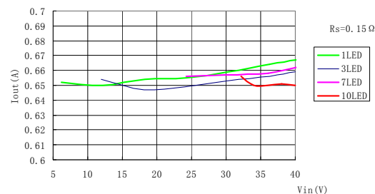
Output current variation with output Voltage L=47\mu\text{H} , R_s=0.15\Omega\text{hm}
