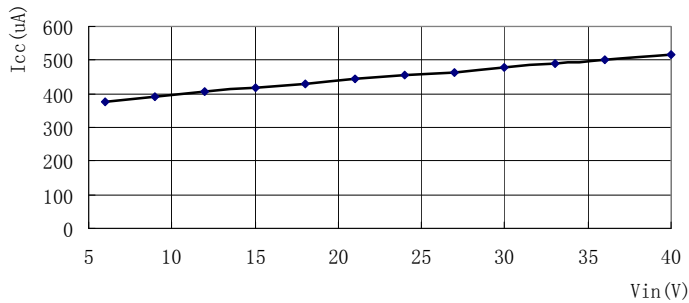
Operating Supply Current vs. Vin
