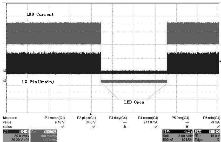
LED open circuit protection V_{in}=24VDC , L=47\mu H , R_s=0.30\Omega
