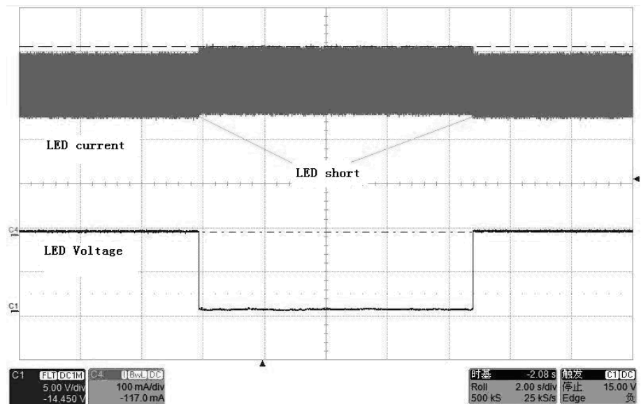
LED short circuit protection V_{in}=24VDC , L=47\mu H , R_s=0.30\Omega
