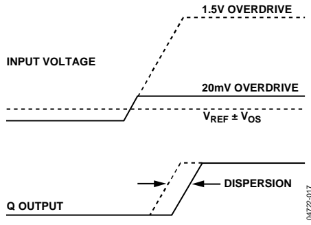
Figure 18. Propagation Delay Dispersion
