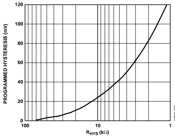
Figure 13. Comparator Hysteresis vs. R_{HYS}
