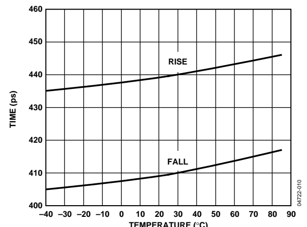
Figure 10. ADCMP553 Rise/Fall Time vs. Temperature
