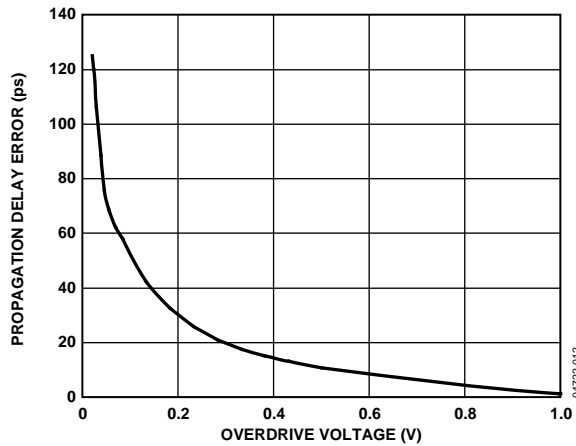
Figure 12. Propagation Delay vs. Overdrive Voltage
