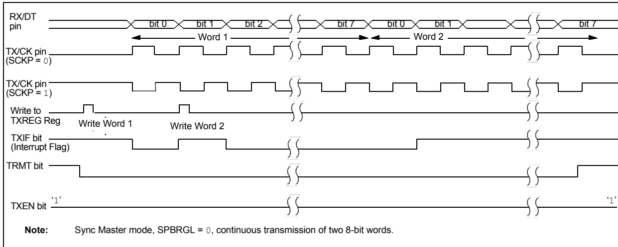
FIGURE 21-10: SYNCHRONOUS TRANSMISSION
