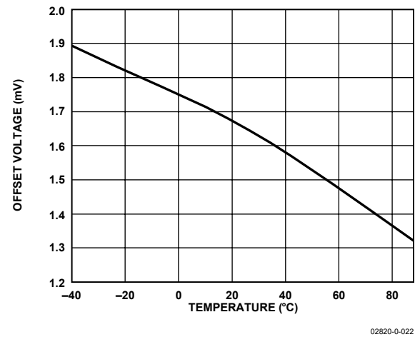
Figure 13. Input Offset Voltage vs. Temperature
