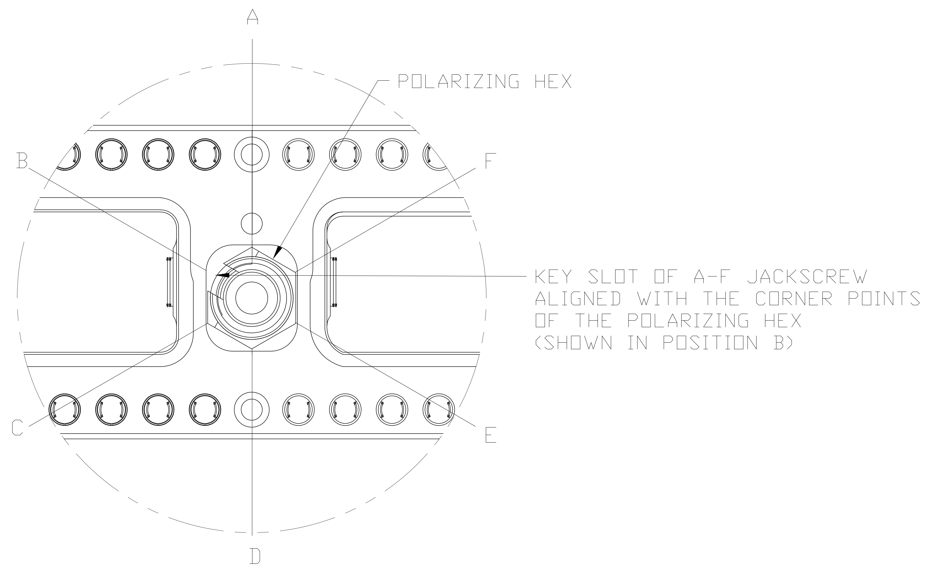
DETAIL A -JACKSCREW KIT ASSEMBLED
