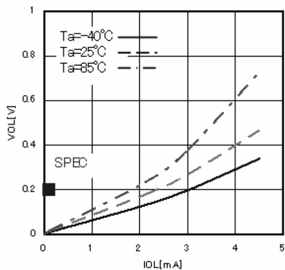
Figure 4. L output voltage V_{OL-IOL} ( V_{CC}=1.8\text{V} )
