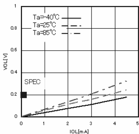
Figure 5. L output voltage V_{OL-IOL} ( V_{CC}=2.5\text{V} )
