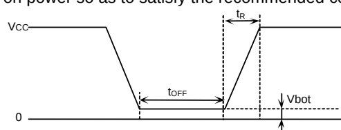
Figure 54. Rise waveform diagram
