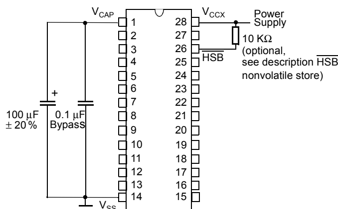
Figure 1: Automatic STORE Operation Schematic Diagram
