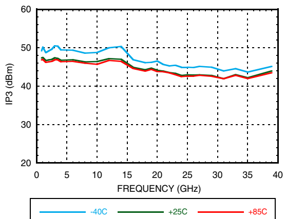
Input IP3 vs. Temperature
