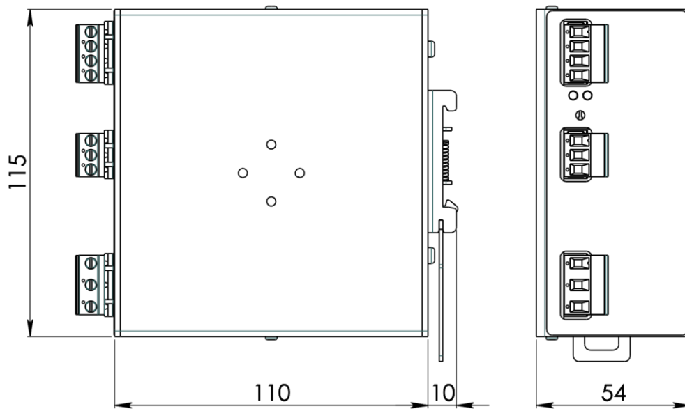
Figure 1. Mechanical Drawing
