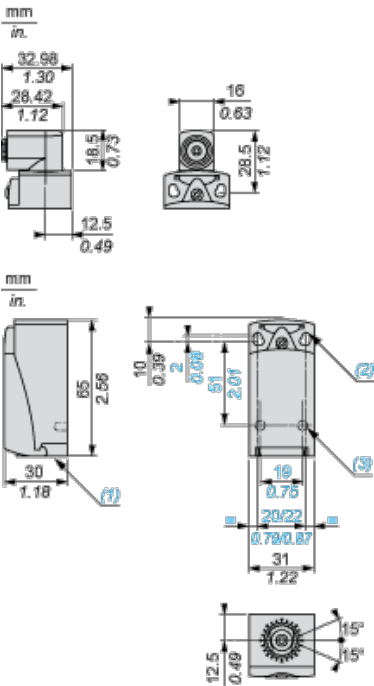
(1) Tapped entry for Pg 11 cable gland
