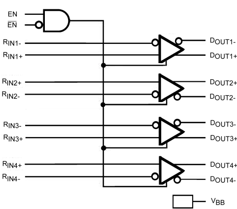
Functional Diagram
