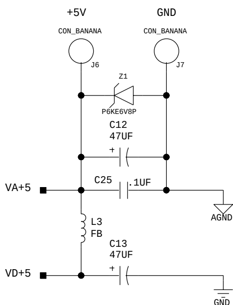
Figure 9. Power Supply
