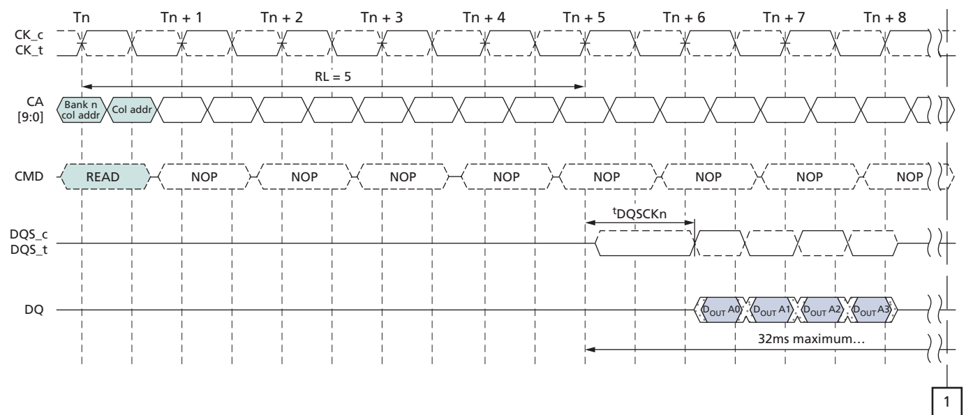
Figure 26: t_{DQSCKDL} Timing
