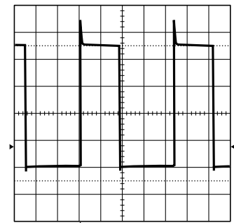
Figure 17. Transient Response
