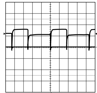
Figure 19. Drain Voltage
