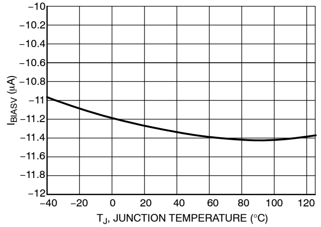
Figure 12. IBIASV at VCC = 15 V, VSNS > VSNSBIASV
