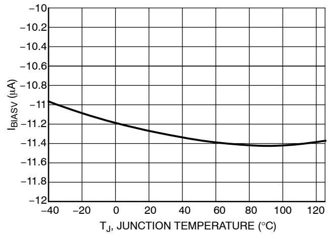
Figure 12. IBIASV at VCC = 15 V, VSNS > VSNSBIASV
