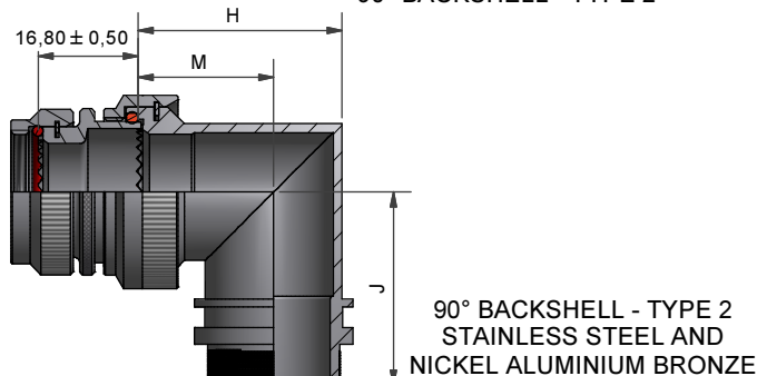
90° BACKSHELL - TYPE 2
